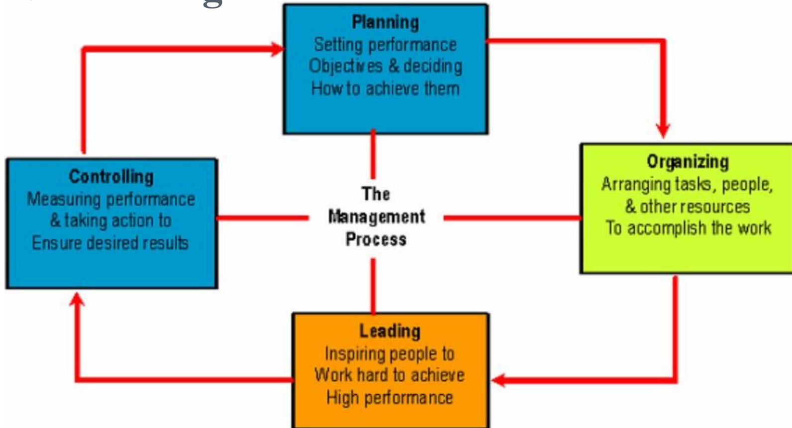
Figure 1.2: Management Functions
